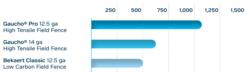
Field Fence Breaking Strength in pounds
