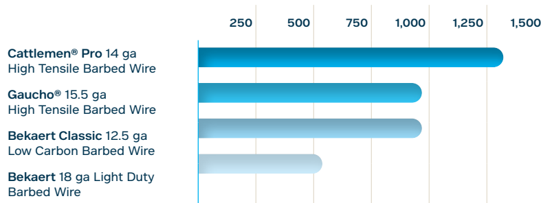
Barbed Wire Breaking Strength in pounds
