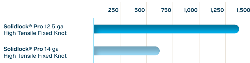
Fixed Knot Fence Breaking Strength in pounds
